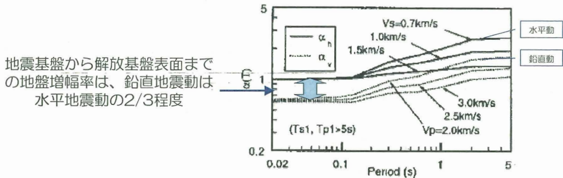
Noda et al (2002) : Response Spectra for Design Purpose of Stiff Structures on Rock Sites, OECD-NEA Workshop on the Relations between Seismological DATA and Seismic Engineering, Oct. 16-18, Istanbul, pp.399-408
